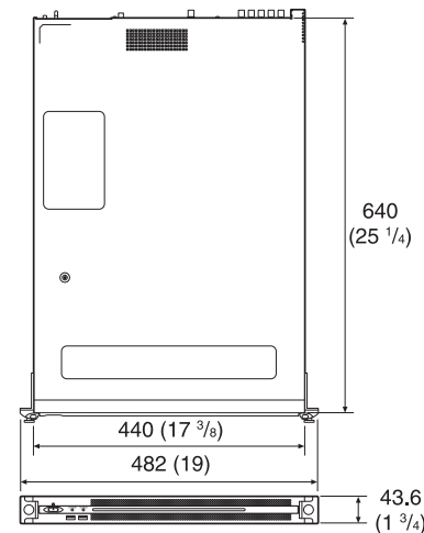
PWS-100MG1/PWS-100RC1
