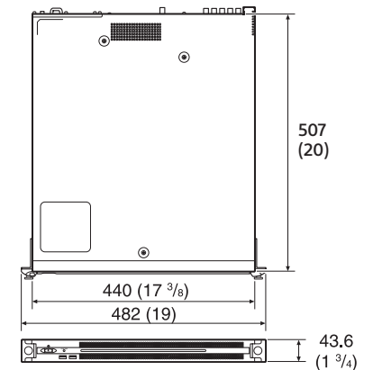
PWS-110PR1/110MG1/110CM1
